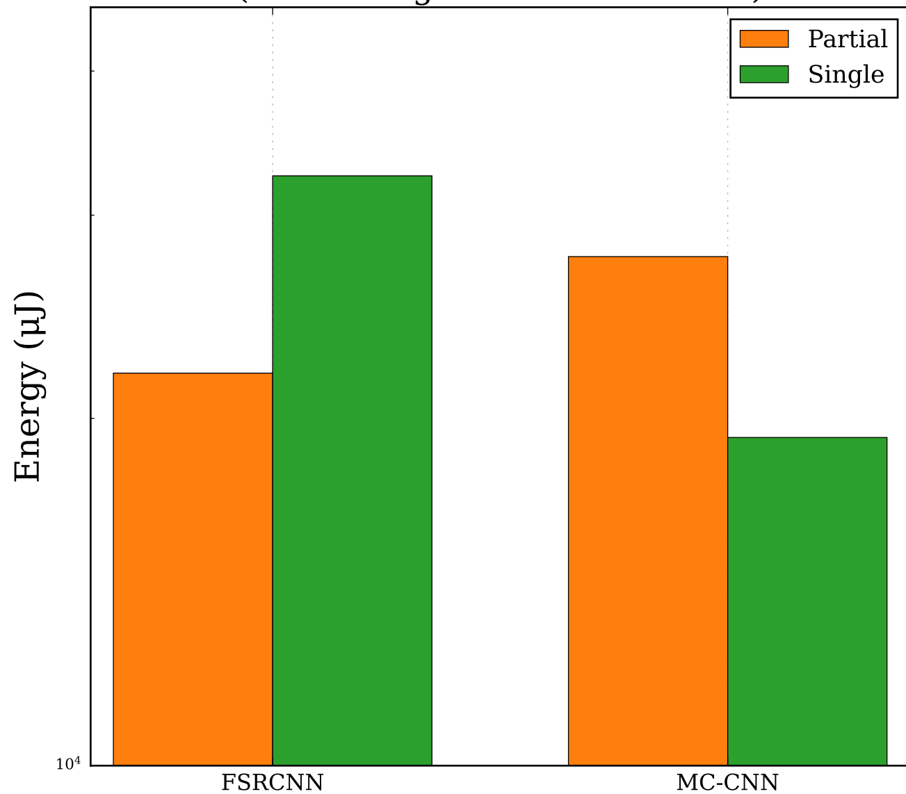
Eyeriss (2048 PEs, WReg=384) (same wreg for both scenarios)
