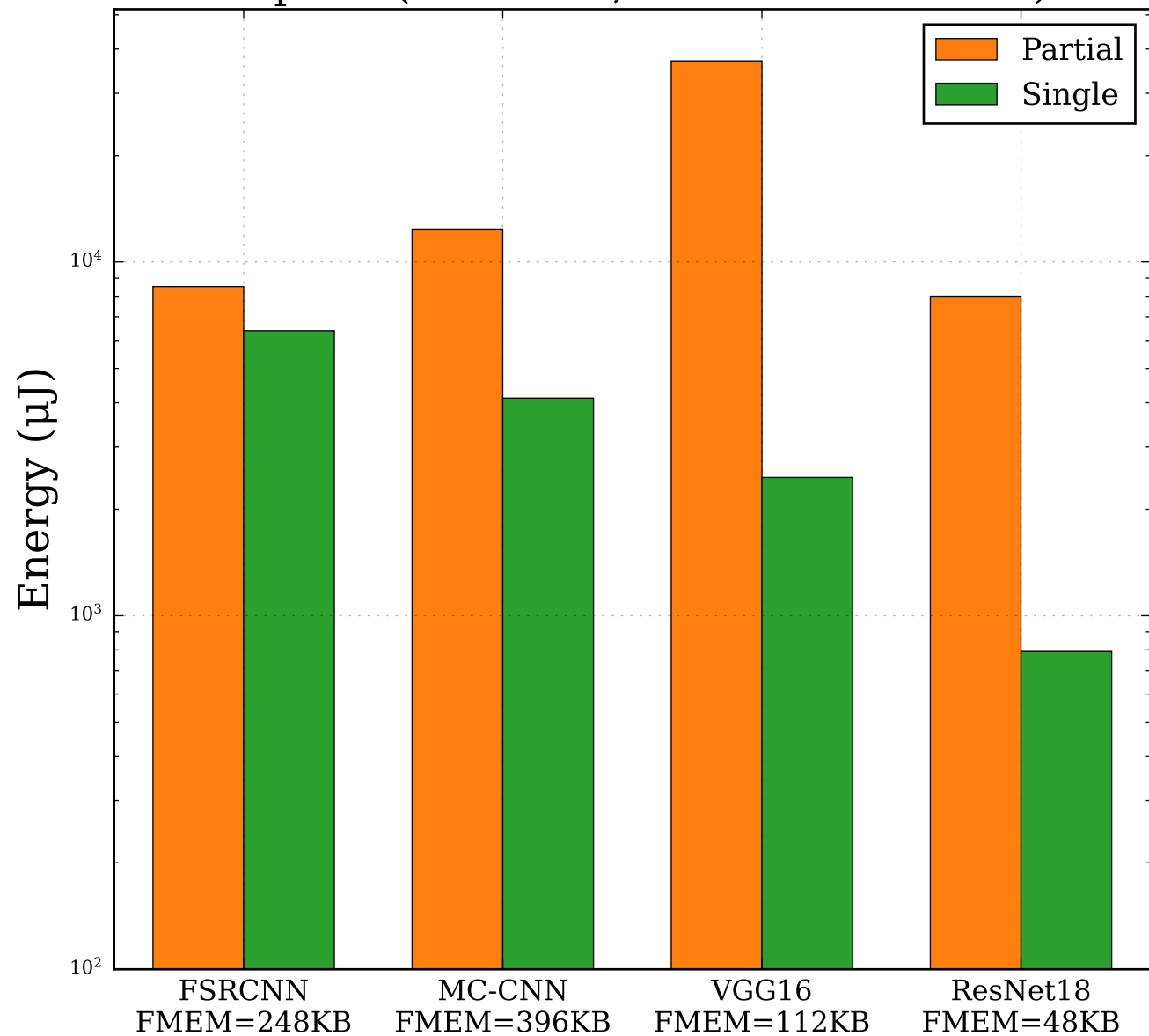
DepFiN (2048 PEs, Partial-Sized Mem)
