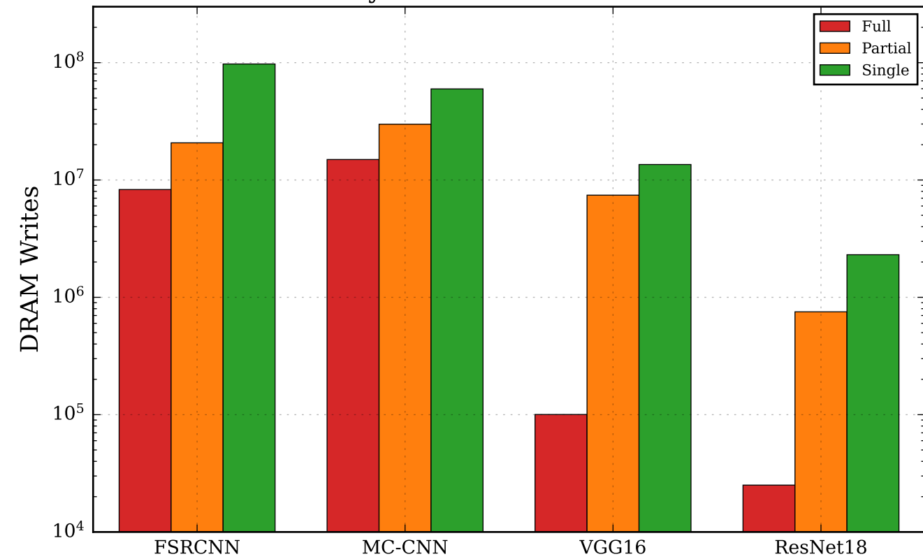
Eyeriss — DRAM Writes
