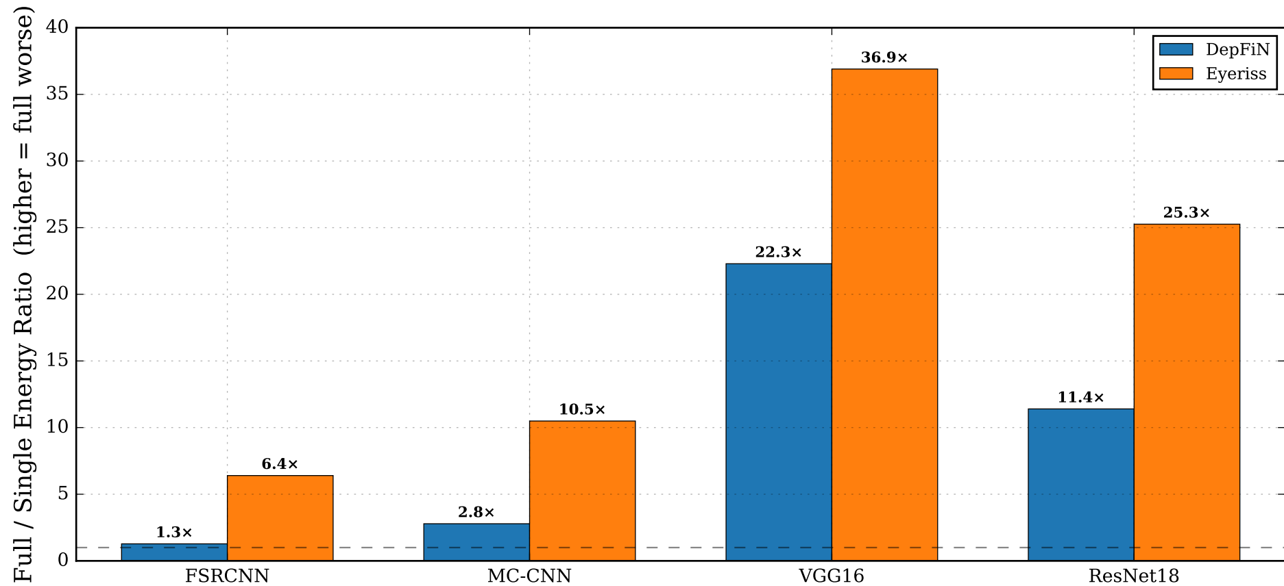
Full-Sized Arch — Full/Single Energy Ratio
