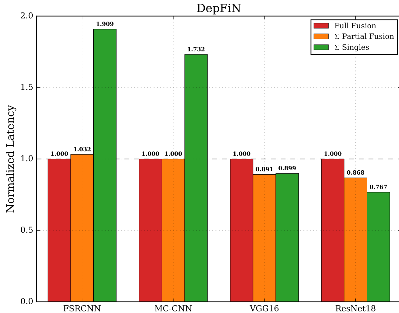
Scenario A — Normalized Latency (Full = 1.0, DRAM = 200 pJ/byte)
