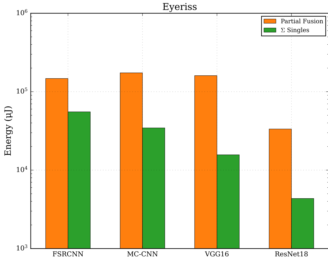
Scenario B — Energy (Partial vs Single, DRAM = 200 pJ/byte)
