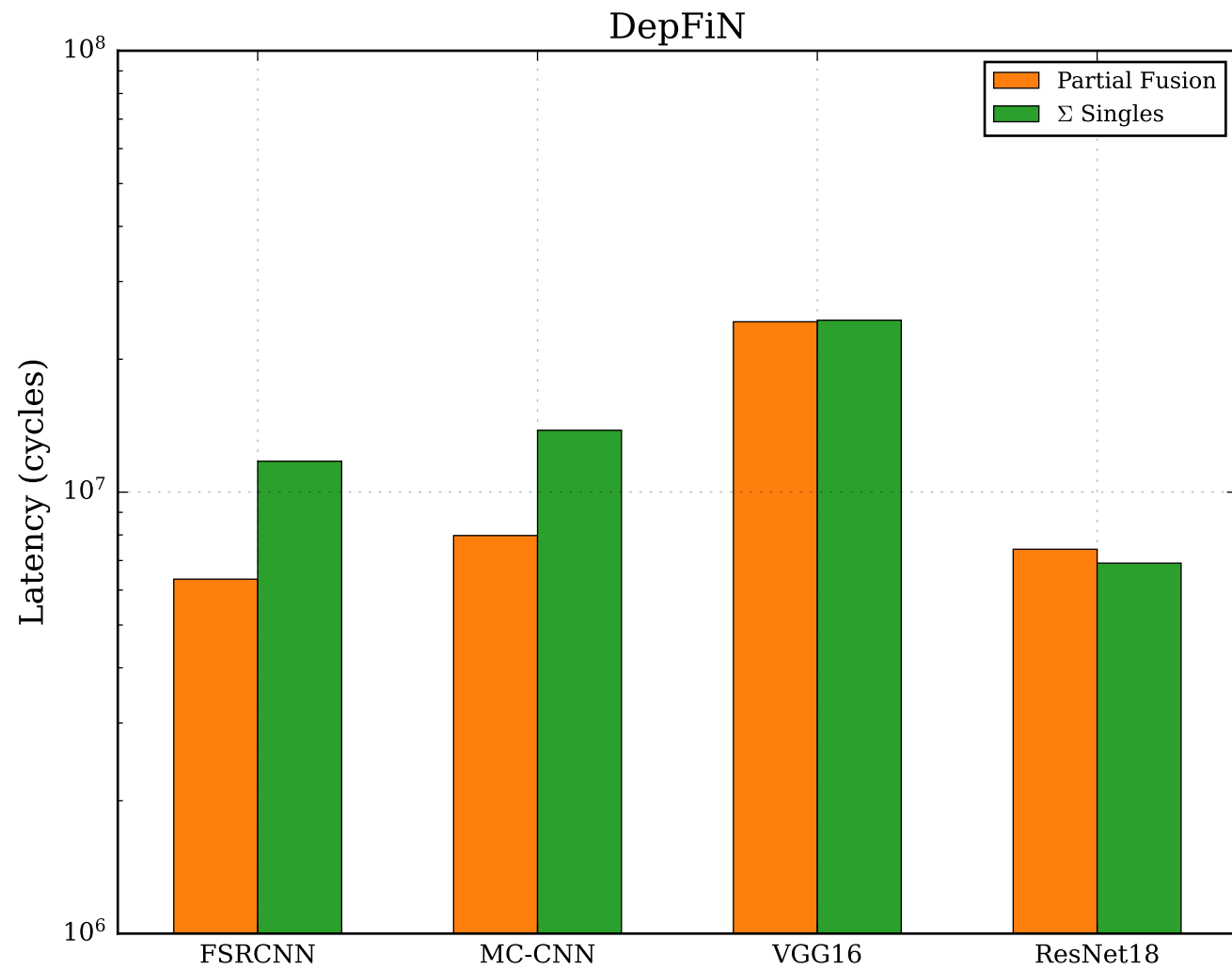
Scenario B — Latency (Partial vs Single, DRAM = 200 pJ/byte)
