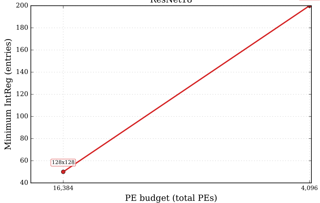
ResNet18
