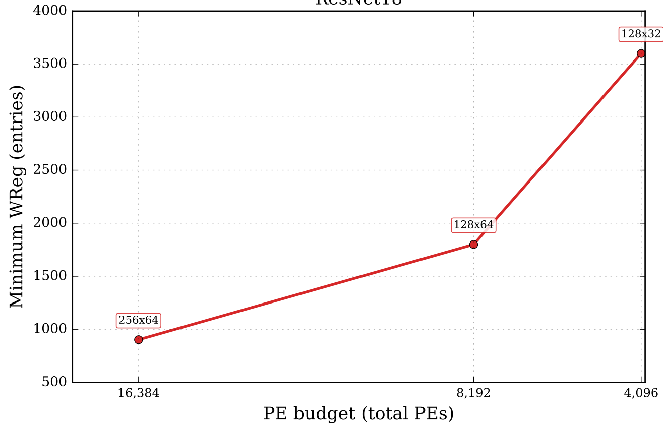
ResNet18
