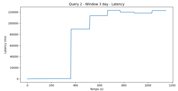
Fig. 14. Latency Query 2 - Window 3 day
