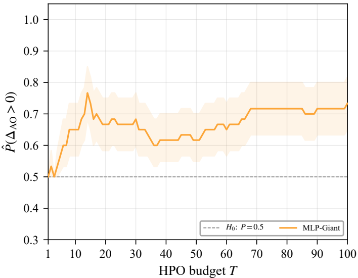
MLP-Giant ( T = 100 )
