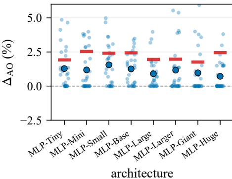
MNIST-1D
