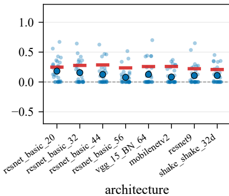
CIFAR-10
