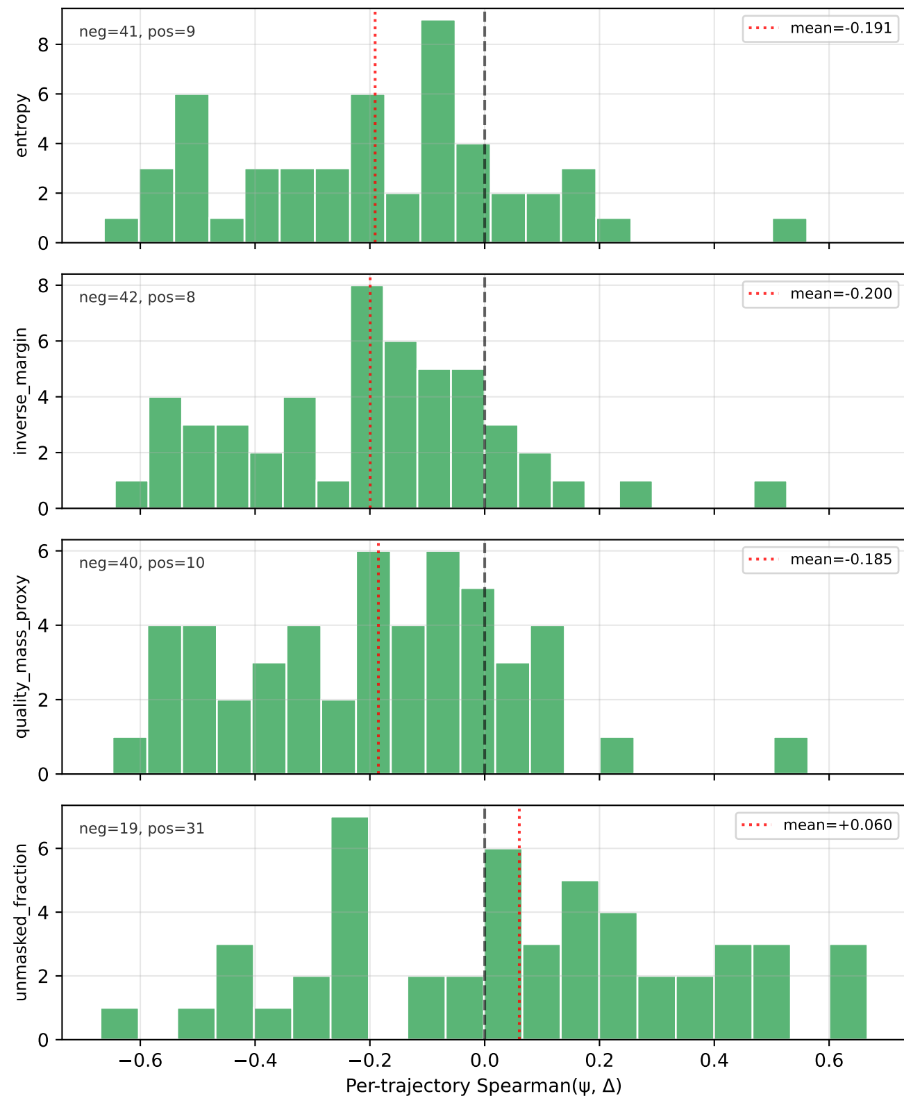
Per-trajectory rank correlation of signal vs \Delta_t
