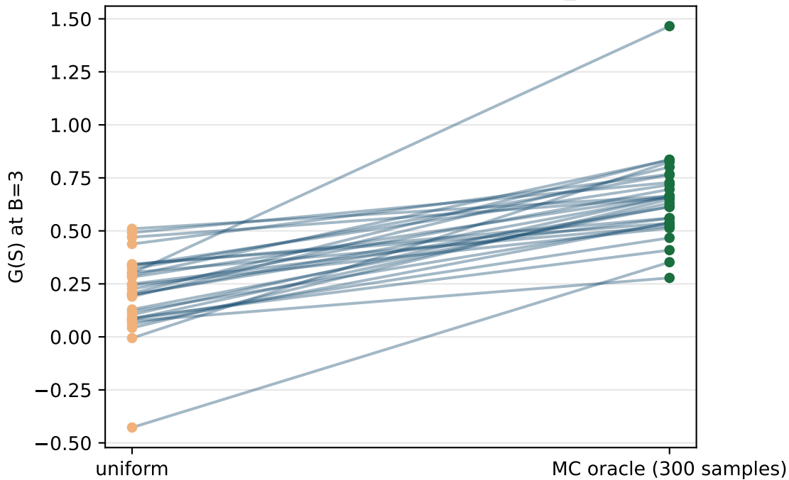
MC-oracle headroom over uniform — B=3 , \Delta_{\text{mean}}=+0.441
