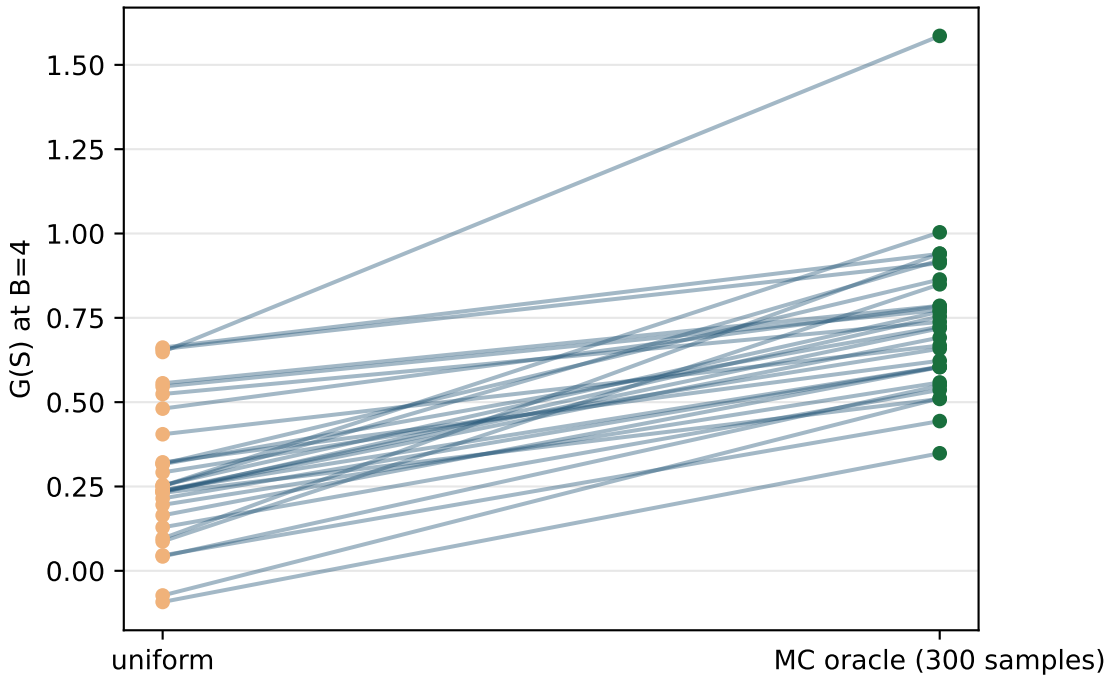
MC-oracle headroom over uniform — B=4 , \Delta_{\text{mean}}=+0.450
