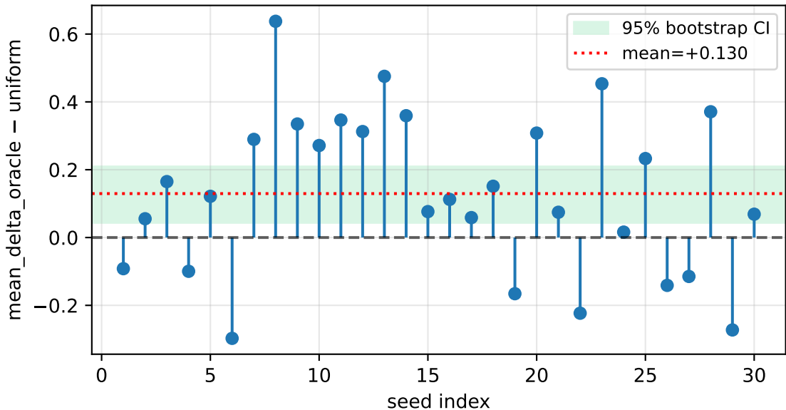
Paired difference — policy='mean_delta_oracle', B=2 — tier T2
