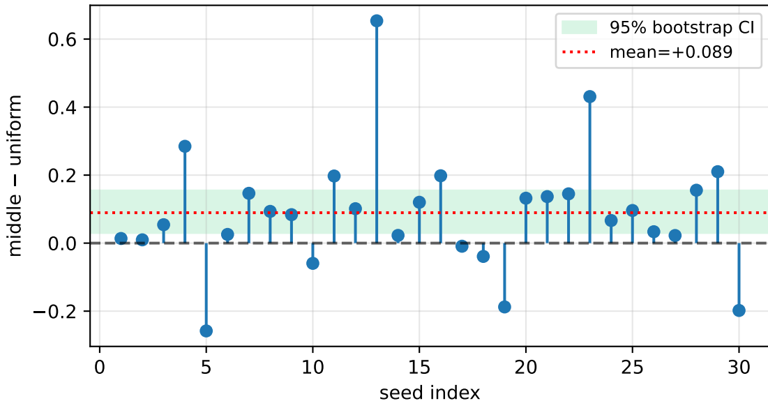
Paired difference — policy='middle', B=2 — tier T2
