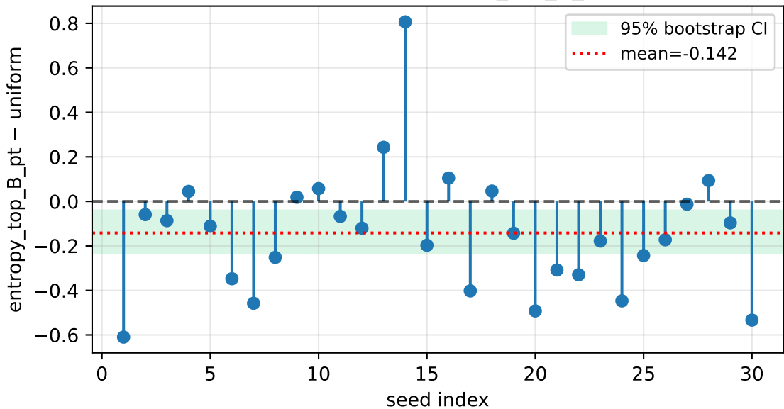
Paired difference — policy='entropy_top_B_pt', B=3 — tier T2
