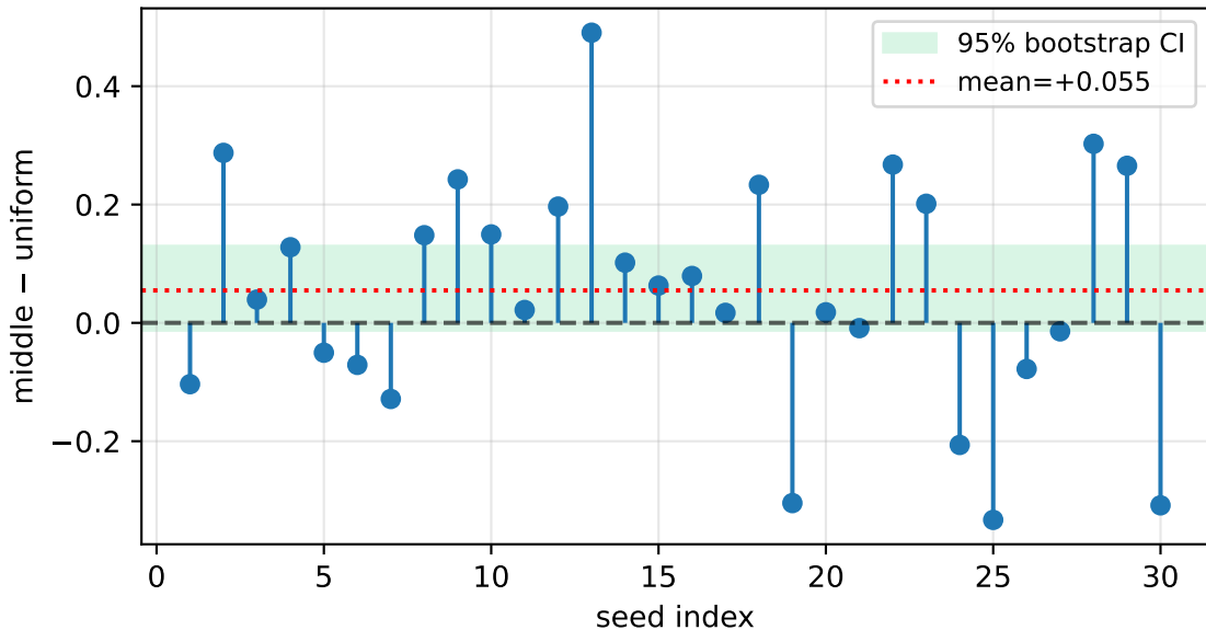
Paired difference — policy='middle', B=3 — tier T3
