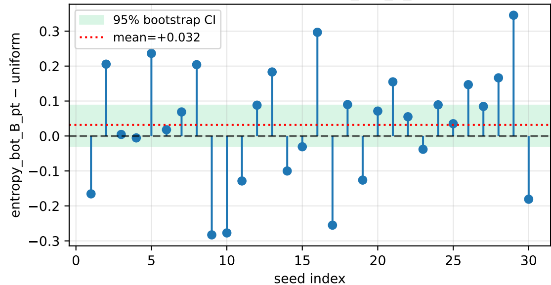
Paired difference — policy='entropy_bot_B_pt', B=4 — tier T3
