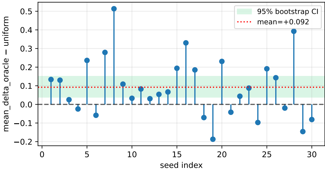
Paired difference — policy='mean_delta_oracle', B=4 — tier T1
