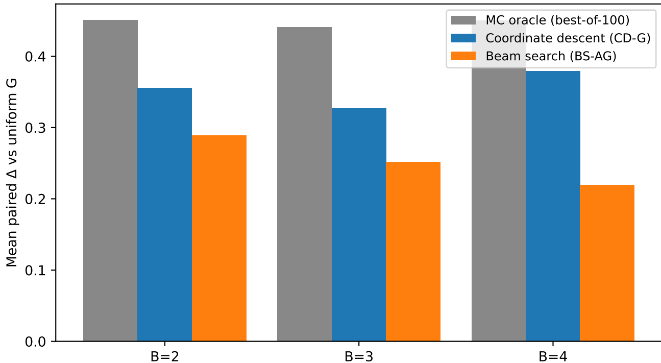
Phase 3a — oracle-gap closure (paired, K=30)
