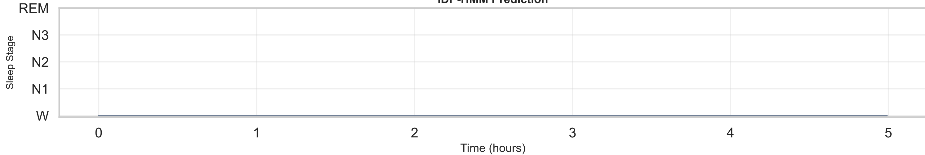
iDP-HMM Prediction
