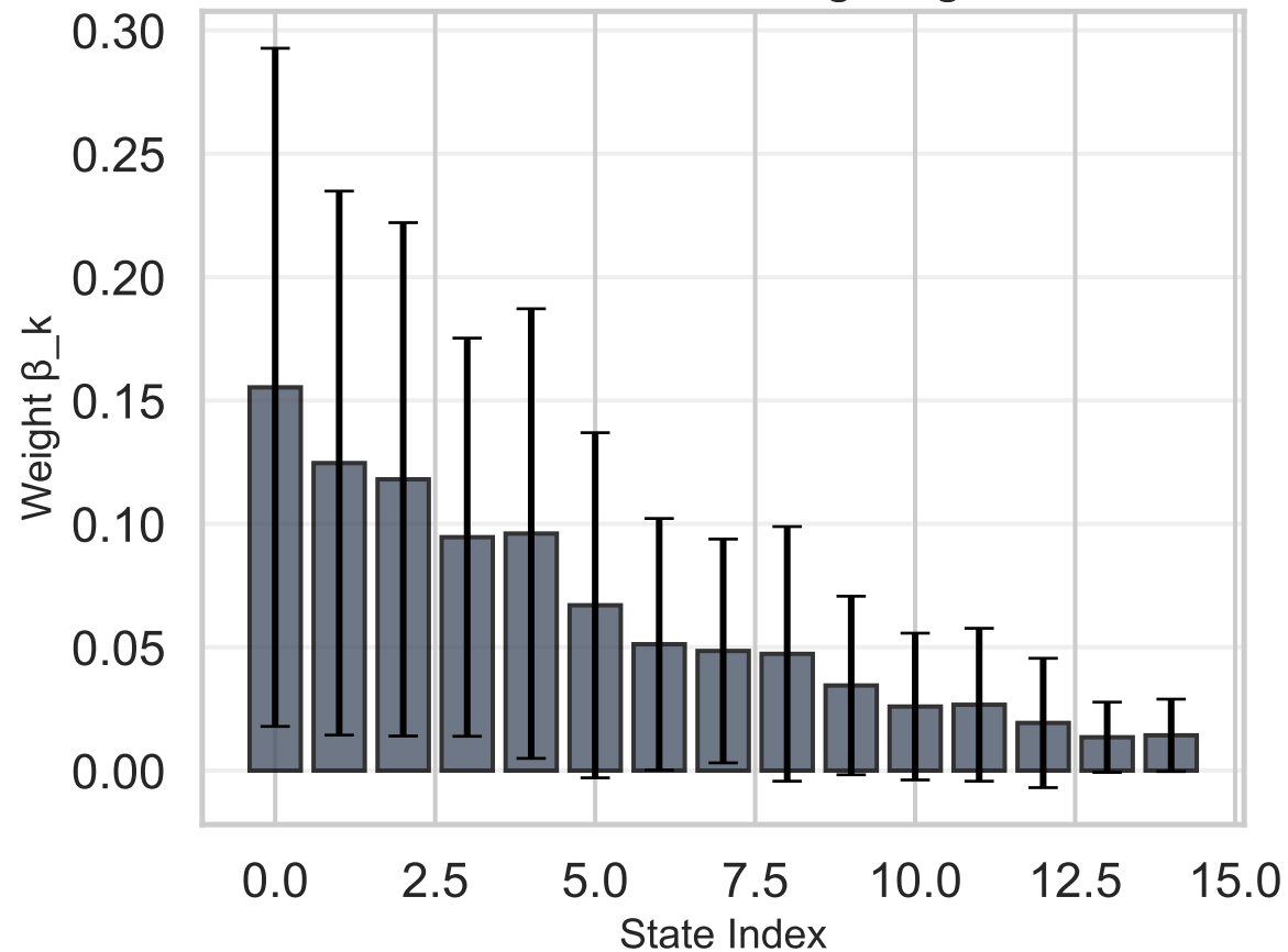
Global Stick-Breaking Weights
