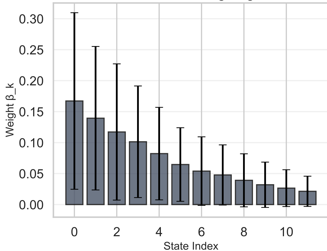
Global Stick-Breaking Weights
