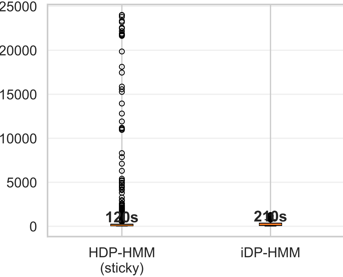
Median Dwell Times
