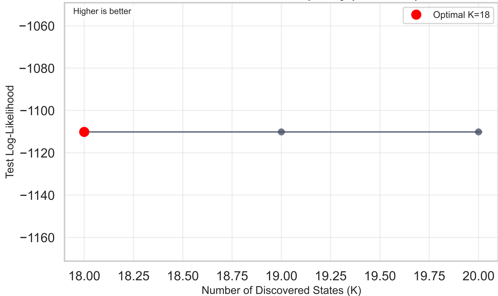
Model Performance vs Complexity (HDP-HMM)
