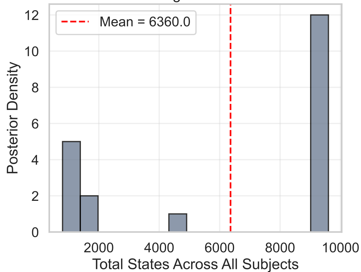
iDP-HMM: Fragmented State Count
