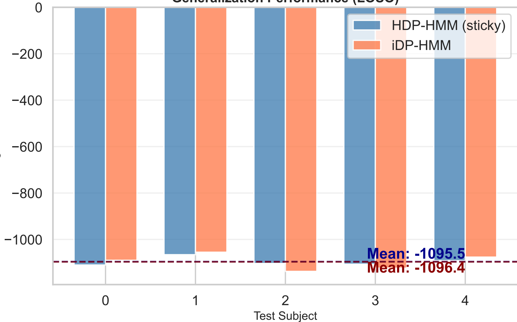
Generalization Performance (LOSO)
