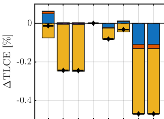
Lifecycle emissions
