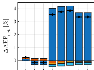
Net AEP
