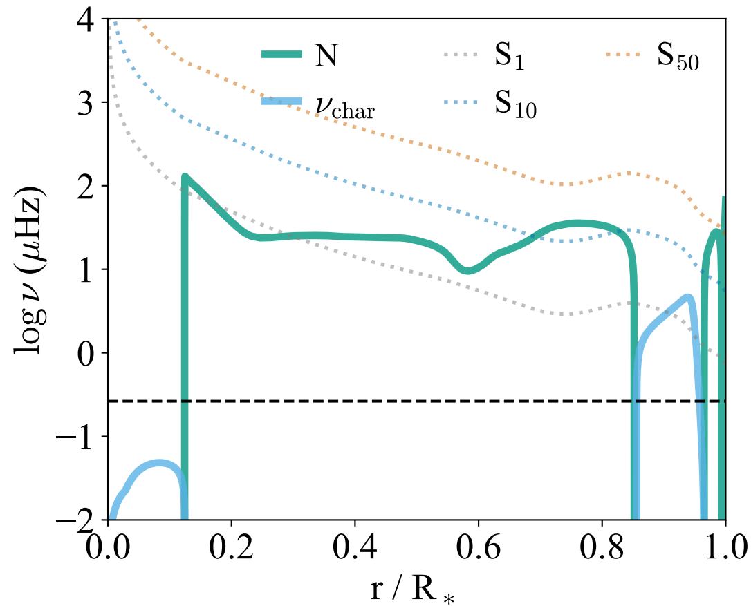
Propagation Diagram for M = 40M_{\odot}
