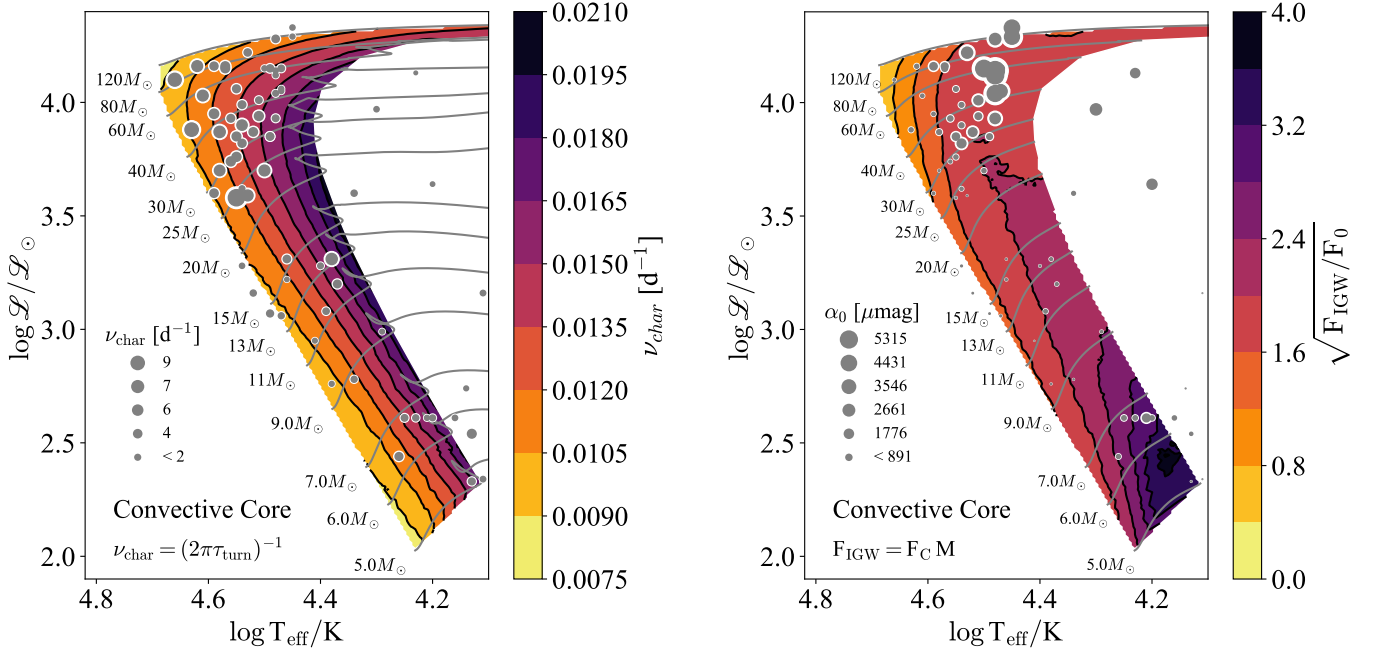
Figure 4. Left panel: Characteristic frequency \nu_{\text{char}} in the convective core as function of the location of stellar models in the spectroscopic H-R diagram. We also show the observed stars with detected photometric variability as grey dots. The area of the dot is proportional to \nu_{\text{char}} . Right panel: Square root of the ratio between the flux of gravity waves launched by the convective core and F_0 = 1/2\rho(r)r^3\omega^2\sqrt{N(r)^2 - \omega^2} , evaluated at the stellar surface. In the absence of damping, this quantity is expected to be proportional to the relative radial displacement (Appendix B) and hence to the relative luminosity fluctuations at the surface. The IGW flux is calculated multiplying the core convective flux by the average convective Mach number in the top pressure scale height of the convective region. We also show the observed stars with detected stochastic, low-frequency photometric variability as grey dots. The area of the dot is proportional to \alpha_0 .
