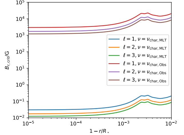
Figure 5. The critical radial magnetic field strength needed to reflect internal gravity waves of different \ell and \nu is shown as a function of fractional depth for a 30M_\odot stellar model at an age of 4 Myr. The frequency \nu_{\text{char,MLT}} is that given by equation (3) but evaluated for the core convection zone instead of the subsurface FeCZ. The frequency \nu_{\text{char,Obs}} is a typical value of 3 \text{ d}^{-1} for the observations.
