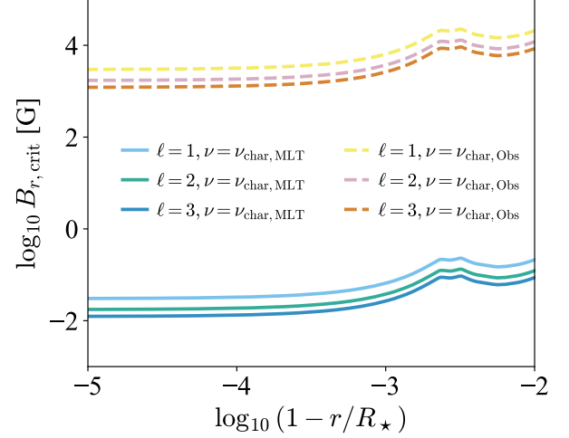
Figure 5. The critical radial magnetic field strength needed to reflect waves of different \ell and \nu is shown as a function of fractional depth for a 30M_\odot stellar model at an age of 4 Myr. The frequency \nu_{\text{char,MLT}} is that given by equation (2) but evaluated for the core convection zone instead of the subsurface FeCZ. The frequency \nu_{\text{char,Obs}} is a typical value of 3 \text{ d}^{-1} for the observations.
