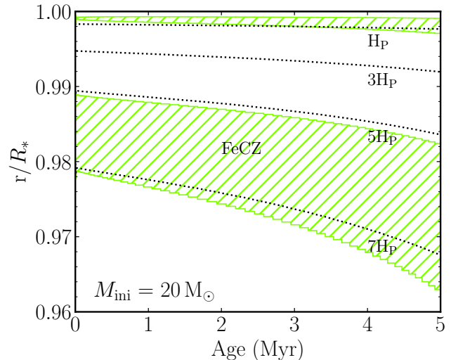
Figure 1. Evolution of the normalized radial location of the FeCZ in a 20M_{\odot} model during the main sequence (first 5 Myr of evolution). The HeCZ is also visible very close to the surface. Locations of P(r)/P(R_*) = e^n for n = [1, 3, 5, 7] are also shown and labelled as nH_P .
