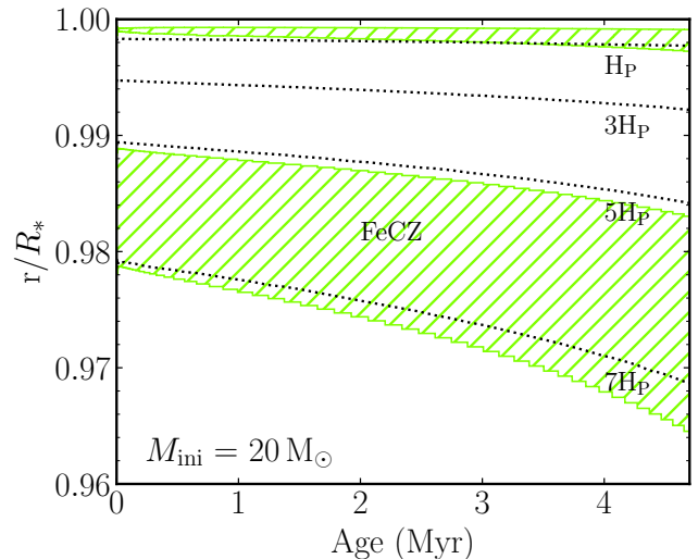
Figure 1. Evolution of the normalized radial location of the FeCZ in a 20M_{\odot} model during the main sequence (first 4.7 Myr of evolution). The FeCZ is also visible very close to the surface. Locations of P(r)/P(R_*) = e^n for n = [1, 3, 5, 7] are also shown and labelled as nH_P .
