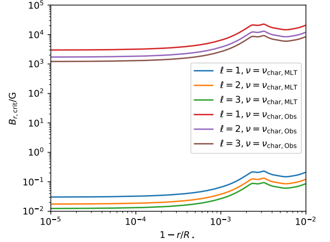
Figure 5. The critical radial magnetic field strength needed to reflect waves of different \ell and \nu is shown as a function of fractional depth for a 30M_{\odot} stellar model at an age of 4 Myr. The frequency \nu_{\text{char,MLT}} is that given by equation (2) but evaluated for the core convection zone instead of the subsurface FeCZ. The frequency \nu_{\text{char,Obs}} is a typical value of 3 \text{ d}^{-1} for the observations.
