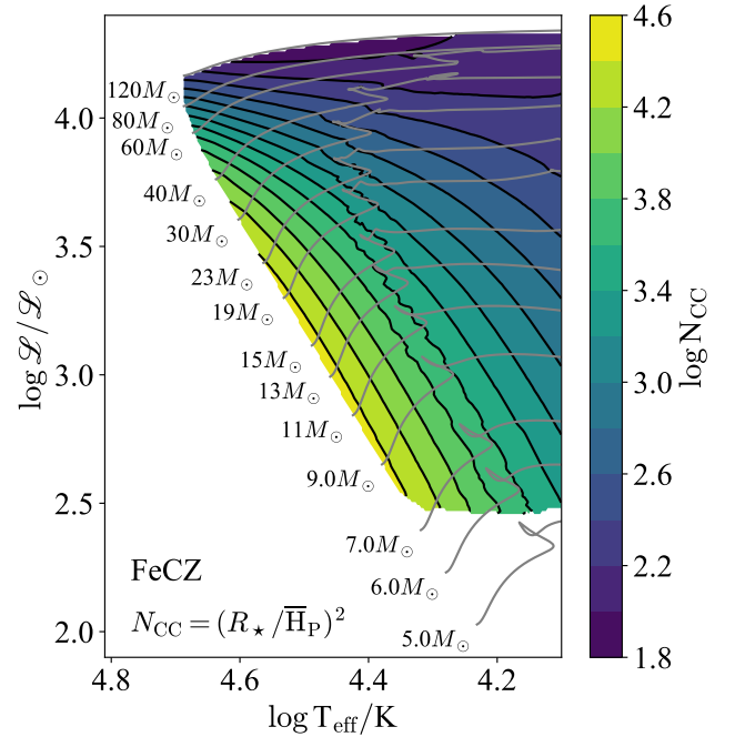
Figure 6. Number of convective cells in the FeCZ. This was calculated using the average pressure scale height in the FeCZ.
