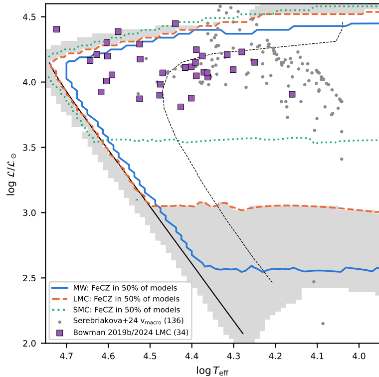
LMC: grey = LMC models without an FeCZ (v2, \omega = 0 )
