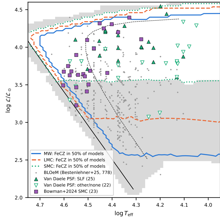
SMC: grey = SMC models without an FeCZ (v2, \omega = 0 )
