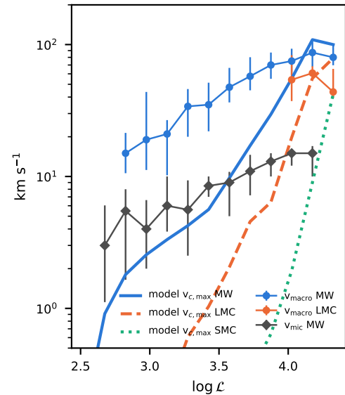
(a) velocities, \log T_{\text{eff}} > 4.3
