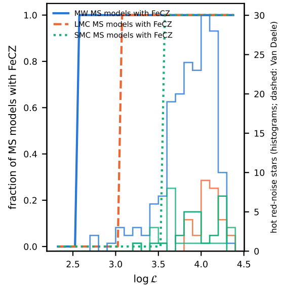
(d) where the FeCZ exists vs where the data are
