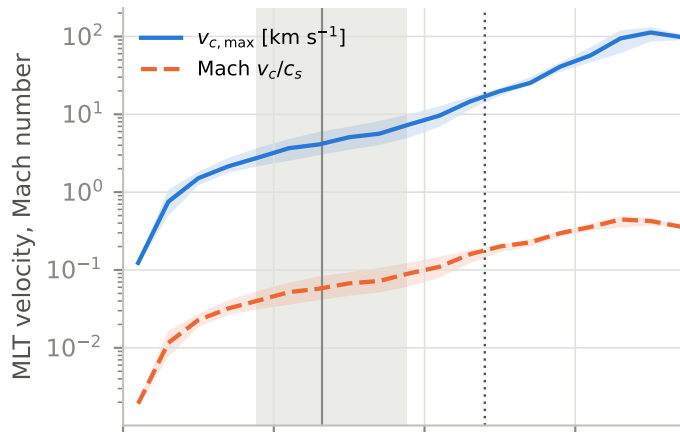
FeCZ regime parameters, MESA v2 (MW, non-rotating, hot M5); 3D models of Schultz+2023 at right
