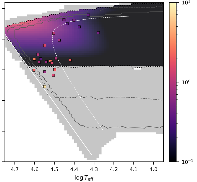
SMC: 3.4 \times \text{model } v_c vs v_{\text{char}} (N = 23)
