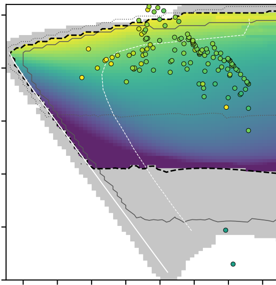
LMC: model v_{c, \max} ; stars with SLF light curves
