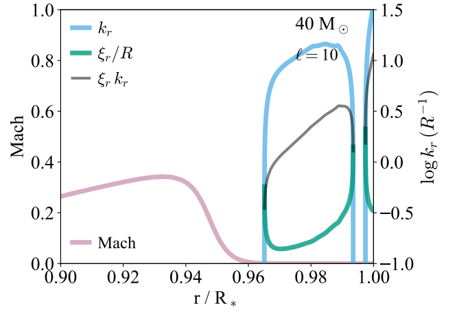
Figure 8. Properties of waves launched by the FeCZ in a 40M_\odot model. The plot shows the outer 10% of the star in radial coordinate.
