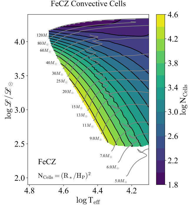
Figure 6. Expected number of convective cells in the FeCZ. This is calculated assuming the size of convective cells is about the average pressure scale height in the FeCZ
