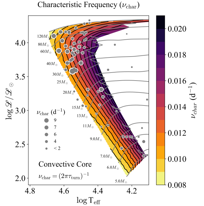
Figure 10. Characteristic frequency \nu_{\text{char}} in the convective core as function of the location of stellar models in the spectroscopic HRD. We also show the observed stars with detected stochastic photometric variability as grey dots. The size of the dot is proportional to \nu_{\text{char}} .
