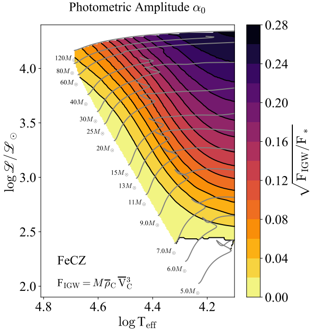
Figure 5. Relative flux of IGWs launched by the FeCZ. The IGWs flux is calculated multiplying the convective flux in the FeCZ by the average convective Mach number, calculated in the top pressure scale height of the convective region.
