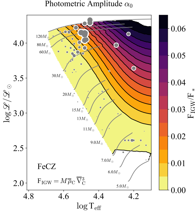
Figure 11. Flux of gravity waves launched by the FeCZ. This is calculated multiplying the convective flux in the FeCZ by the average convective Mach number (this is calculated in the top pressure scale height of the convective region). We also show the observed stars with detected stochastic photometric variability as grey dots. The size of the dot is proportional to \alpha_0 .
