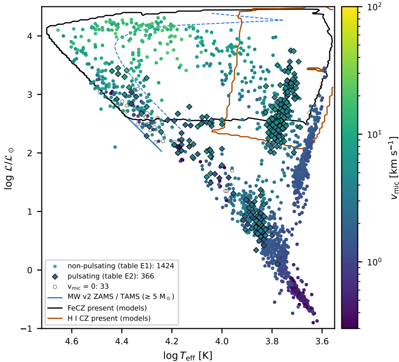
Microturbulence, Markova+2025 (N = 1823)
