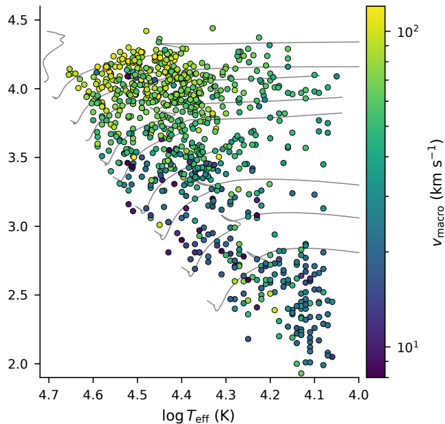
b IACOB macroturbulence sample (N=832)
