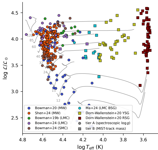
a Red-noise samples (N=342)
