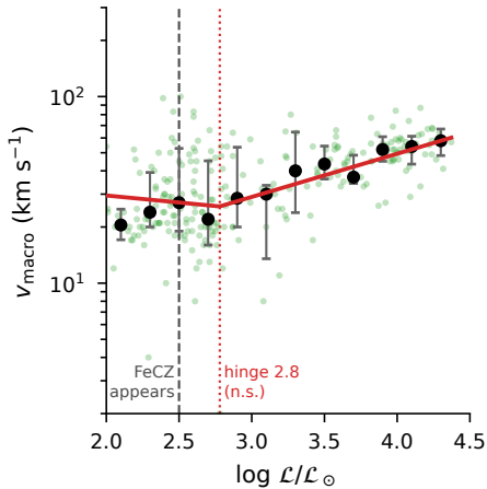
b v_{\text{macro}}, 4.0 < \log T_{\text{eff}} \leq 4.3 (N=253)
