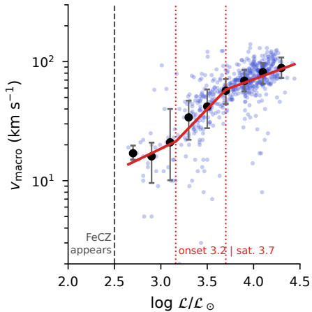
a v_{\text{macro}}, \log T_{\text{eff}} > 4.3 (N=579)
