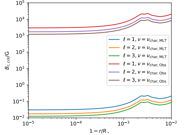
Figure 5. The critical radial magnetic field strength needed to reflect waves of different \ell and \nu is shown as a function of fractional depth for a 30M_\odot stellar model at an age of 4 Myr. The frequency \nu_{\text{char,MLT}} is that given by equation (2) but evaluated for the core convection zone instead of the subsurface FeCZ. The frequency \nu_{\text{char,Obs}} is a typical value of 3 \text{ d}^{-1} for the observations.
