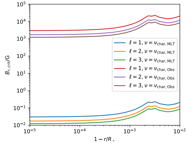
Figure 4. The critical radial magnetic field strength needed to reflect waves of different \ell and \nu is shown as a function of fractional depth for a 30M_\odot stellar model at an age of 4 Myr. The frequency \nu_{\text{char,MLT}} is that given by equation (2) but evaluated for the core convection zone instead of the subsurface FeCZ. The frequency \nu_{\text{char,Obs}} is a typical value of 3\text{d}^{-1} for the observations.
