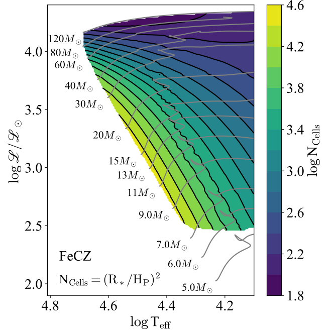
Figure 3. Expected number of convective cells in the FeCZ. This is calculated assuming the size of convective cells is about the average pressure scale height in the FeCZ
