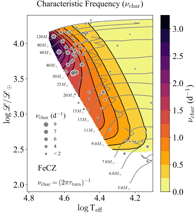
Figure 7. Characteristic frequency \nu_{\text{char}} in the FeCZ as a function of the location of stellar models in the spectroscopic H-R Diagram. We also show the observed stars with detected stochastic photometric variability as grey dots. The size of the dot is proportional to \nu_{\text{char}} .
