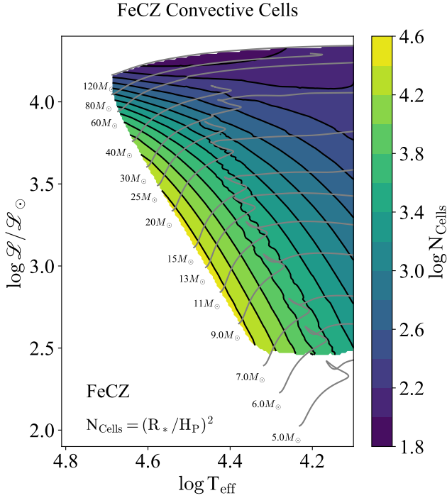
Figure 3. Expected number of convective cells in the FeCZ. This is calculated assuming the size of convective cells is about the average pressure scale height in the FeCZ
