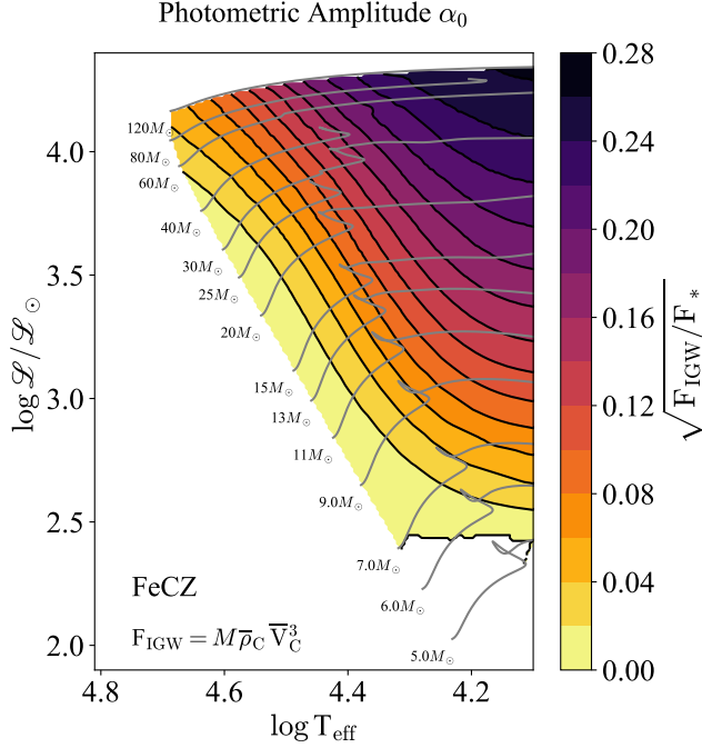
Figure 2. Relative flux of IGWs launched by the FeCZ. The IGWs flux is calculated multiplying the convective flux in the FeCZ by the average convective Mach number, calculated in the top pressure scale height of the convective region.
