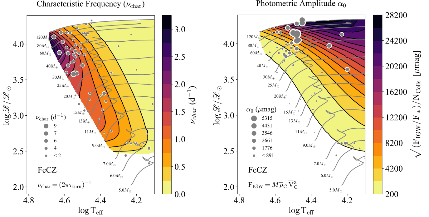
Figure 4. Left panel: Characteristic frequency \nu_{\text{char}} in the FeCZ as a function of the location of stellar models in the spectroscopic H-R Diagram. We also show the observed stars with detected stochastic photometric variability as grey dots. The size of the dot is proportional to \nu_{\text{char}} . Right panel: Luminosity fluctuations expected due to IGWs launched by the FeCZ. This scales with the square root of the relative IGWs flux, with a correction factor accounting for the likely scale of the perturbation. We assumed uncorrelated perturbations at the surface with typical scale of a convective cell, so a correction factor \sim 1/\sqrt{N_{\text{Cells}}} . The IGWs flux is calculated multiplying the convective flux in the FeCZ by the average convective Mach number (this is calculated in the top pressure scale height of the convective region. The agreement is pretty good, considering that uncertainties of a factor of 2 in the MLT \alpha parameters for these regions result in a factor of 20 in luminosity perturbations). We also show the observed stars with detected stochastic photometric variability as grey dots. The size of the dot is proportional to \alpha_0 .
