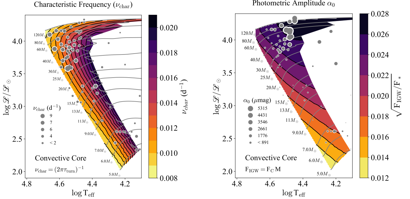
Figure 5. Left panel: Characteristic frequency \nu_{\text{char}} in the convective core as function of the location of stellar models in the spectroscopic HRD. We also show the observed stars with detected stochastic photometric variability as grey dots. The size of the dot is proportional to \nu_{\text{char}} . Right panel: Flux of gravity waves launched by the convective core. This is calculated multiplying the convective flux in the core by the average convective Mach number (this is calculated in the top pressure scale height of the convective region). We also show the observed stars with detected stochastic photometric variability as grey dots. The size of the dot is proportional to \alpha_0 .
