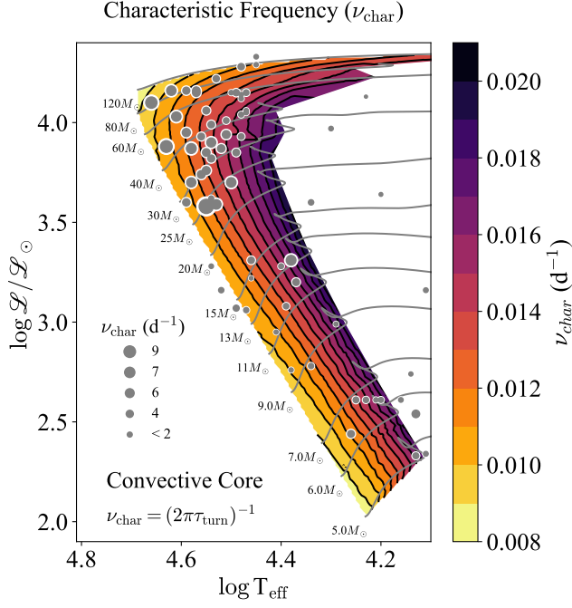
Figure 6. Characteristic frequency \nu_{\text{char}} in the convective core as function of the location of stellar models in the spectroscopic HRD. We also show the observed stars with detected stochastic photometric variability as grey dots. The size of the dot is proportional to \nu_{\text{char}} .
