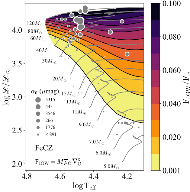
Figure 10. Flux of gravity waves launched by the FeCZ. This is calculated multiplying the convective flux in the FeCZ by the average convective Mach number (this is calculated in the top pressure scale height of the convective region). We also show the observed stars with detected stochastic photometric variability as grey dots. The size of the dot is proportional to \alpha_0 .
