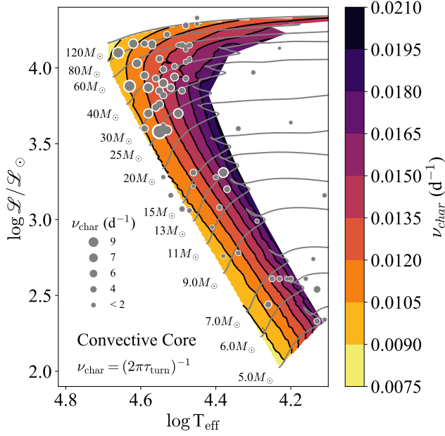
Figure 9. Characteristic frequency \nu_{\text{char}} in the convective core as function of the location of stellar models in the spectroscopic HRD. We also show the observed stars with detected stochastic photometric variability as grey dots. The size of the dot is proportional to \nu_{\text{char}} .
