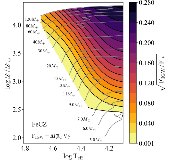
Figure 2. Relative flux of IGWs launched by the FeCZ. The IGWs flux is calculated multiplying the convective flux in the FeCZ by the average convective Mach number, calculated in the top pressure scale height of the convective region.
