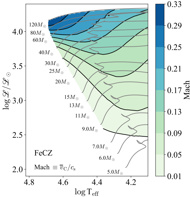
Figure 4. Mach number in the FeCZ.
