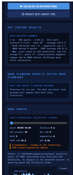
Figure 6: GNSS processing controls and planning results.
