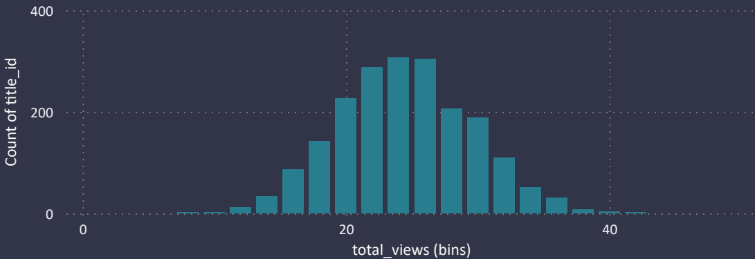
Count of title_id by total_views (bins)
