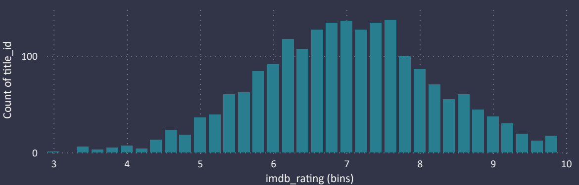
Count of title_id by imdb_rating (bins)
