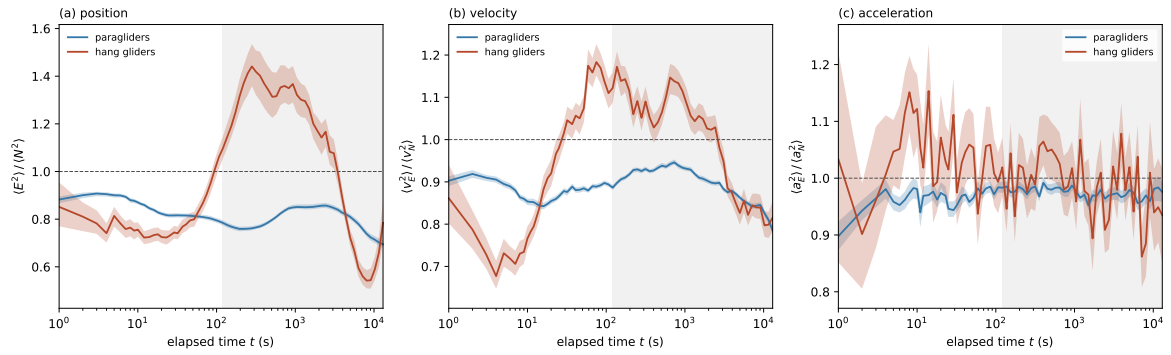
Figure 3.5. The per-component variance ratio read off three quantities rather than one, by discipline: (a) displacement from take-off, (b) velocity, (c) acceleration, all at the same lags and under the same coverage rule. Median and 10% to 90% band over the cluster bootstrap of Sec. 2.8, which resamples whole take-off-site and day groups. The shaded span is the fitted window 120 s to 13,021 s; the panels stop at its upper end, past which fewer than one flight in seven answers a lag. Panel (a) reproduces Fig. 2.14. Unity is isotropy, and the ratio approaches it as the motion is differentiated.
