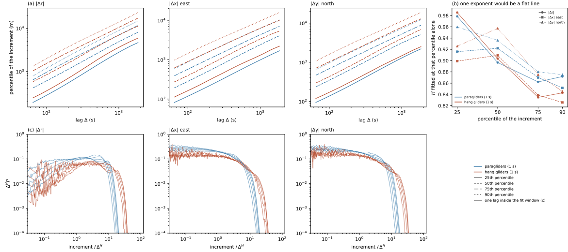
Figure 3.4. The exponent read from the distribution of the increments. All seven panels use each discipline’s fastest native cadence, 1 s, where the histograms hold the most increments. (a) The 25th, 50th, 75th and 90th percentiles against lag, log–log, over the fit window 60 s to 2,000 s, one column for the modulus |\Delta \mathbf{r}| and one for each horizontal component. Four parallel lines would mean one exponent describes every part of that column’s distribution. (b) The slope of each of those four lines, fitted separately, with the modulus and the two components overlaid in one panel. A flat line would mean the same thing as in (a). All three fall from the 25th percentile to the 90th, so the disagreement is not a property of one direction. (c) The histograms behind each column of (a), rescaled by \Delta^H , one curve per lag inside the fit window and every third lag drawn. H = \alpha_2/2 is not a new fit of these histograms: it is the second-order filtered-variation exponent of Table 3.7, reused here rather than re-measured so that a collapsed panel and a quoted exponent never disagree about what H is. For paragliders that is 1.009 (modulus), 0.996 (east), 1.021 (north), and correspondingly 0.972, 0.958, 0.984 for hang gliders.
