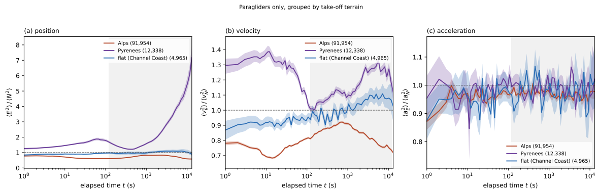
Figure 3.6. The same three quantities, paragliders only, grouped by the orographic box the take-off falls in (Sec. 2.8): the two massifs with the deepest ensembles against the low-relief Channel Coast control. In velocity, panel (b), the two massifs sit on opposite sides of unity and the flat control sits on it; in acceleration, panel (c), the three groups coincide. Bands and shading as in Fig. 3.5.
