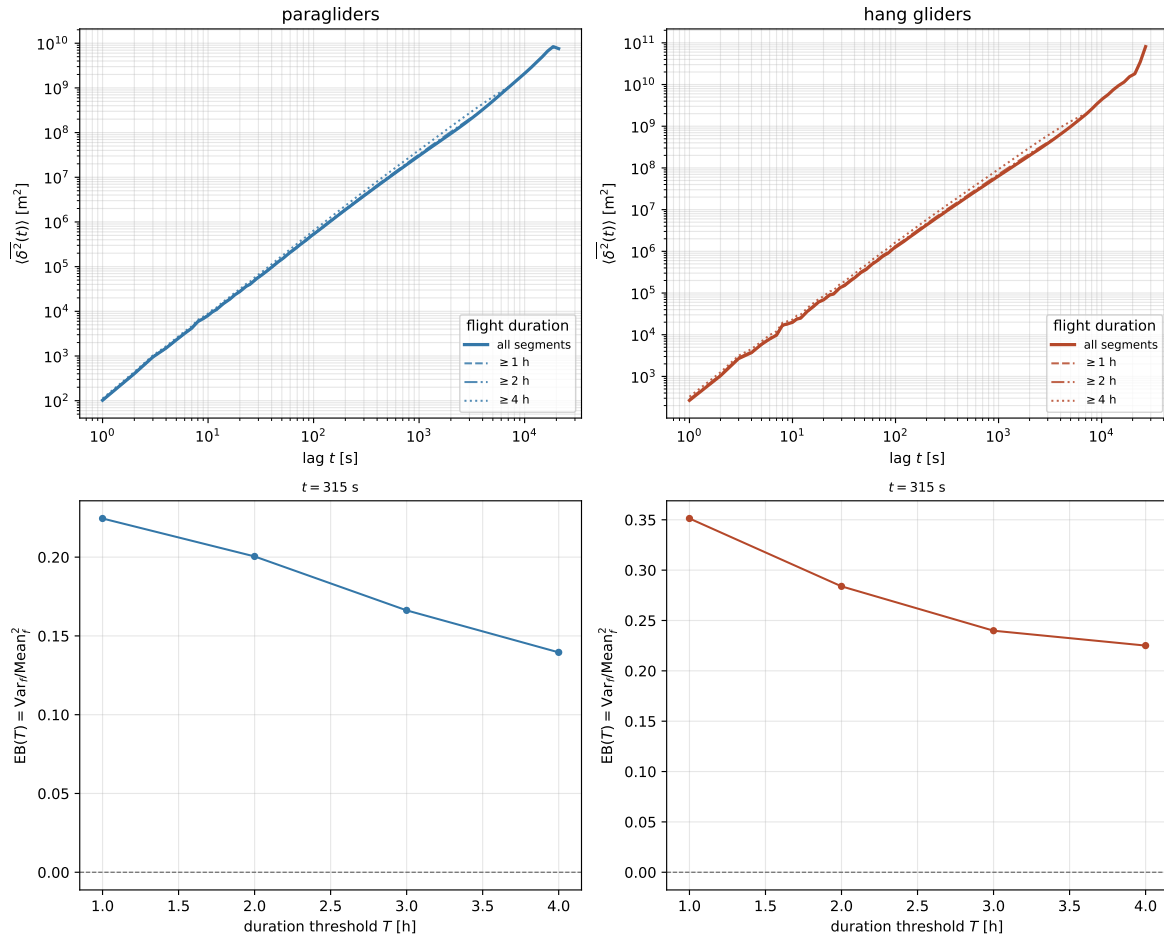
Figure 3.8. Two readings of the same question. (a) The time-averaged MSD of Figure 3.1b ( all segments ) beside its own fixed-duration cohorts, each cut at half its own threshold: coinciding curves would say the time average does not depend on the duration of the record it is read from, and on this archive they separate by tens of per cent, too little to see against eight decades of growth. (b) EB(T) , App. 3.A’s ergodicity-breaking parameter, measured directly from the scatter of each flight’s own time average (Sec. 3.1.2’s V_1 ) rather than proxied by panel (a)’s duration split, at one lag held fixed (315 s) and swept over the duration threshold T : the dependence App. 3.A defines the parameter to test. Zero (dashed) is the ergodic limit, and a curve that falls with T without reaching it weakens the ageing signature without removing it.
