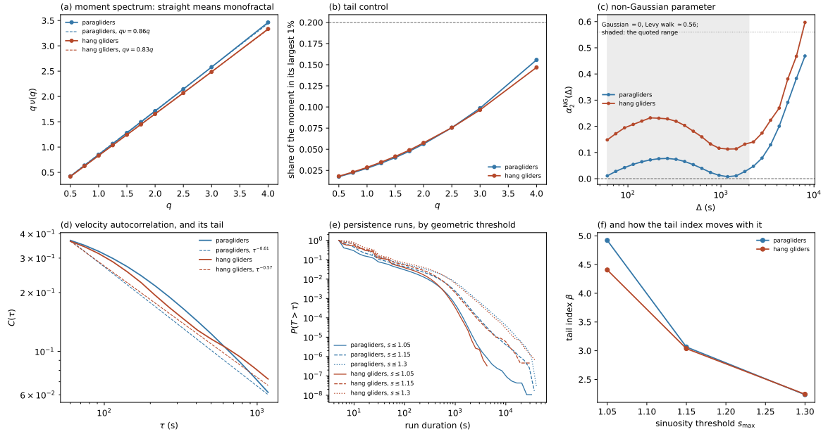
Figure 3.4. What the second moment cannot say. (a) Moment spectrum q\nu(q) , straight line dashed: straight means one exponent for every moment. (b) Share of each moment carried by the largest 1% of increments. (c) Non-Gaussian parameter against lag, Gaussian and Lévy-walk values marked. (d) Velocity autocorrelation, log-log, fitted tail dashed.
