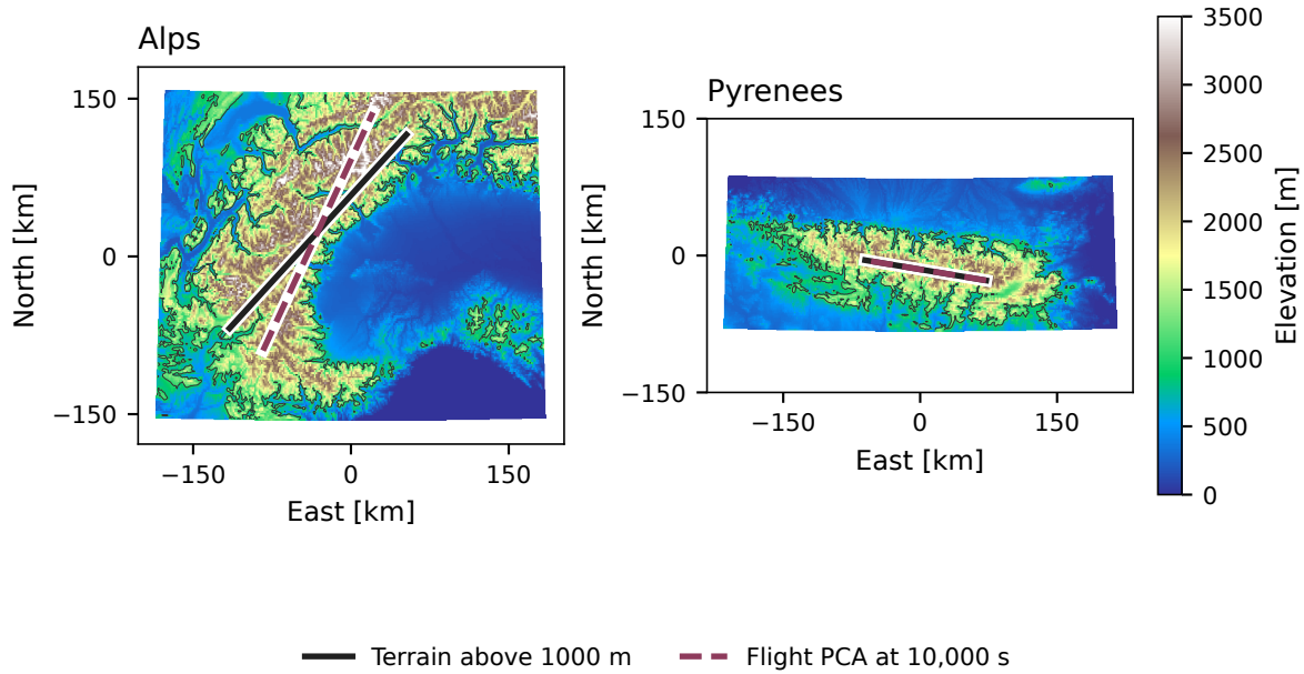
Figure 3.22. Independent terrain orientation compared with the paraglider displacement covariance at 10,000s. Elevation and the 1,000 m contour come from ETOPO 2022 [28]. The solid dark line is the highland-footprint axis; the dashed coloured line is the flight PCA axis, translated to the same centre for comparison. Line lengths carry no displacement or ridge-length information. Map coordinates are kilometres east and north of each box centre.
