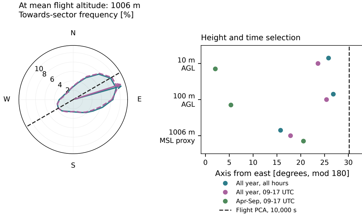
Figure 3.23. ERA5 wind at mean coastal flight altitude and the paraglider PCA at 10,000s. Left: frequencies of air motion towards 15-degree sectors at 1,006 m, for all-year all hours and all-year 09–17 UTC. Speeds below 0.5 \text{ m s}^{-1} are excluded only from the frequency curves; arrows show the vector means using all selected hours. Right: wind axes at flight altitude, approximately above mean sea level, and at 10 and 100 m above ground (AGL). The warm daytime selection is shown as a separate check. The dashed black line is the same flight covariance axis in every comparison.
