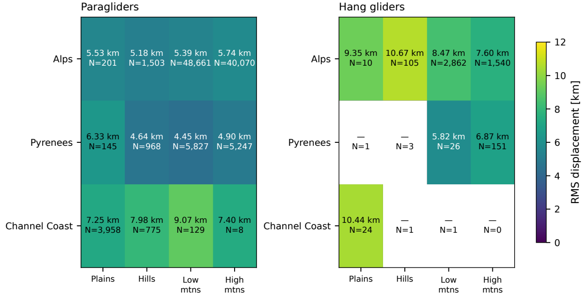
Figure 3.19. Descriptive cross-classification at the requested 1,049 s lag. Each cell gives \sqrt{M_g} and its contributing flight count on available-segment support. Values with fewer than eight flights are suppressed; counts remain visible. The same colour scale applies to both disciplines. These cells carry no calibrated intervals and do not standardise task, weather or pilot identity.
